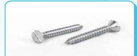
DIN 7972 SLOTTED CSK HD SELF TAPPING SCREW Dia : M2.9-M6.3 Cold Forge Length : 6.5mm-50mm
